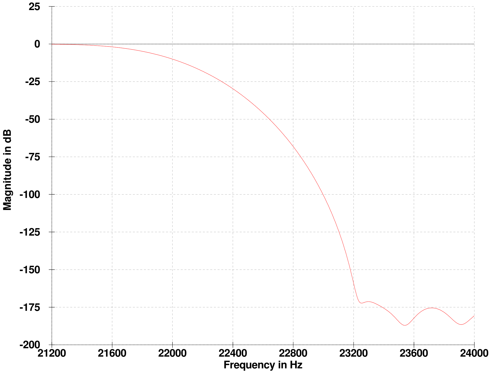
Inphase Filter Frequency Response
