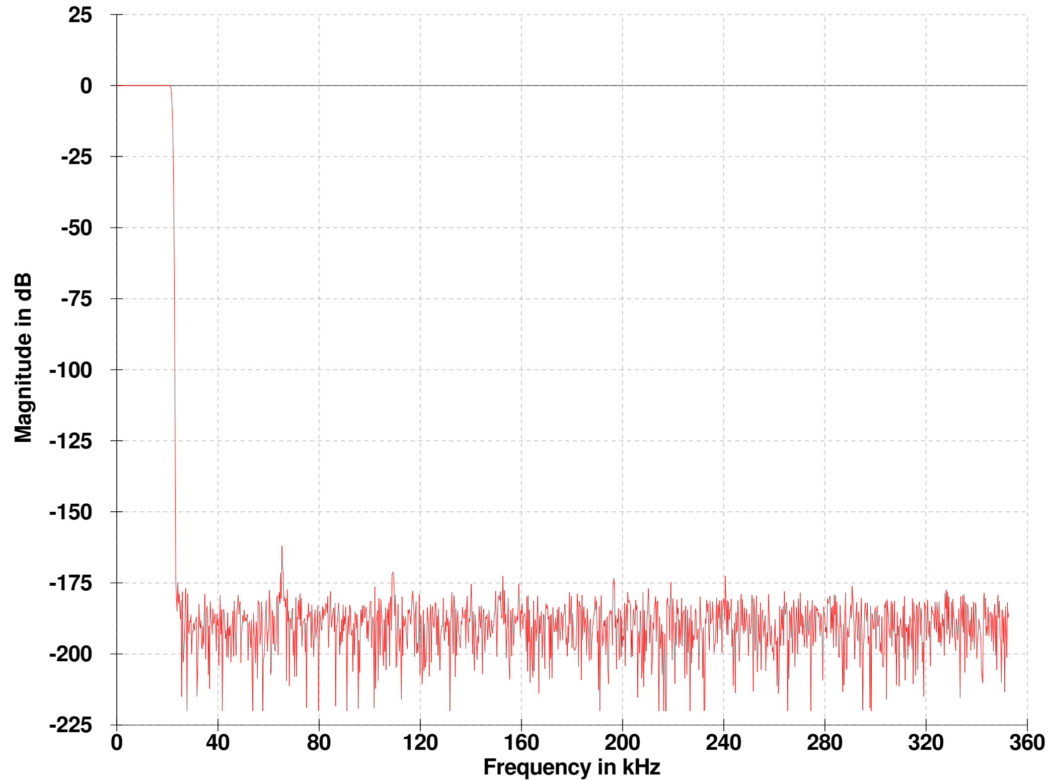
Inphase Filter Frequency Response
