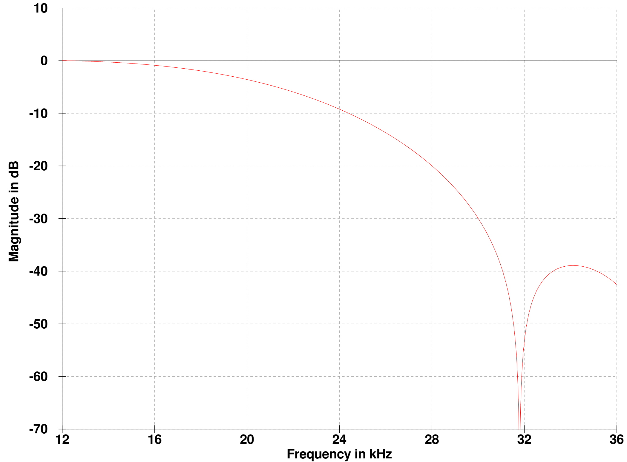
Inphase Filter Frequency Response
